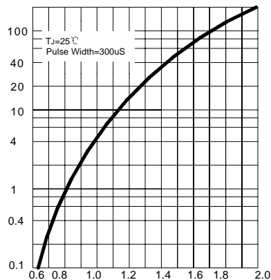
FIG.4 – TYPICAL FORWARD CHARACTERISTIC
