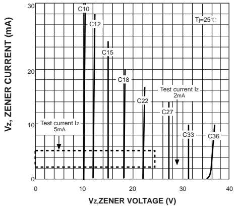
FIG. 3-ZENER BREAKDOWN CHARACTERISTICS
