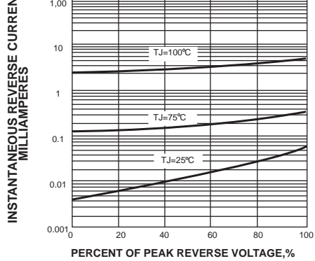
FIG. 4-TYPICAL REVERSE CHARACTERISTICS
